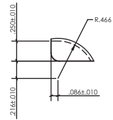
DETAIL SCALE:2:1
